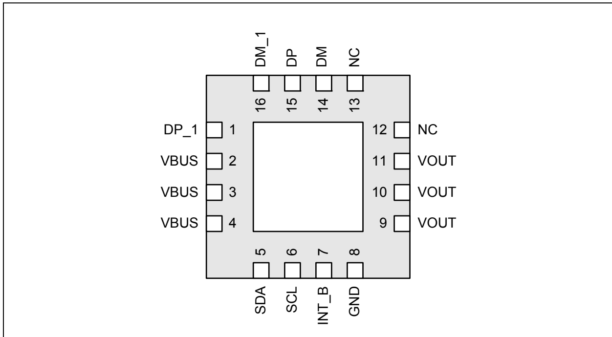
Figure 2.2 QFN Package Diagram (USB3751)
