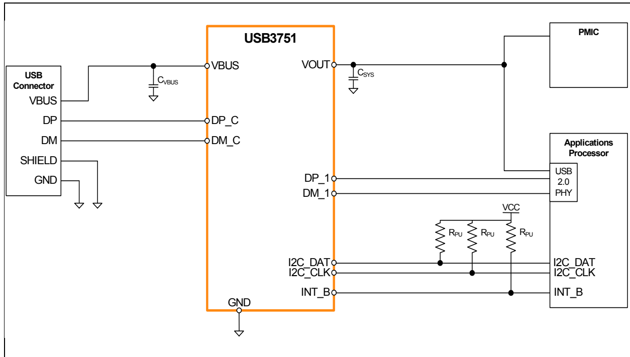
Figure 5.2 USB3751 Device Application Diagram
