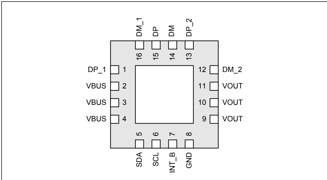
Figure 2.1 QFN Package Diagram (USB3750)
